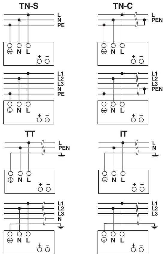
Figure 17 Network types
